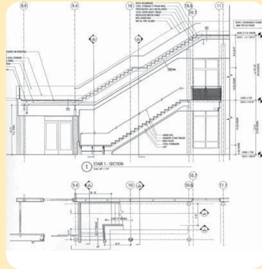
Main Stair Section
